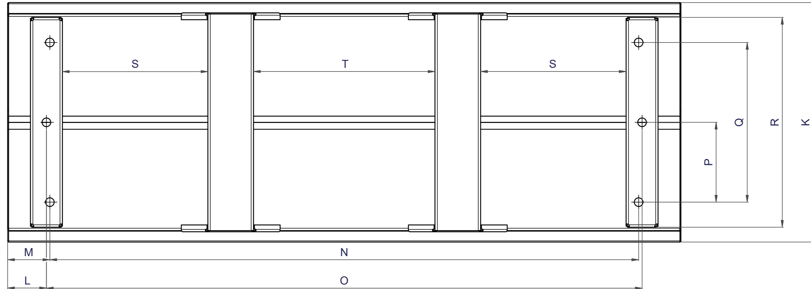
All underframes dimensions (measurements in mm)
